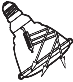
STANDARD Wire supported filament resulting in distorted beam, shorter life
