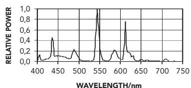
F32T8/SKY-BRITE PLUS® HI LUMEN
