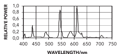
F32T8/841/HI LUMEN- SUPERIOR LIFE®
